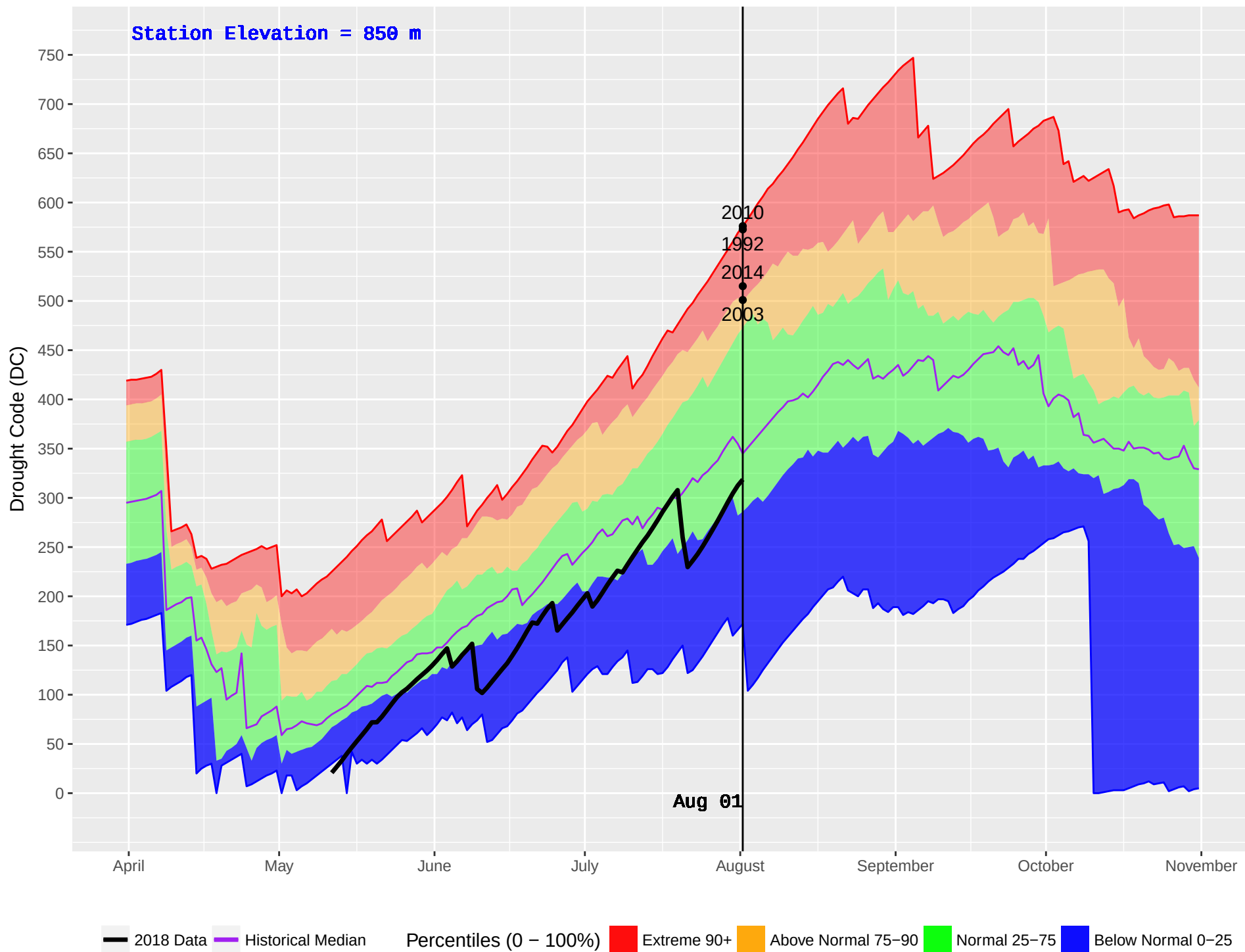
NORTH CHILCO (159) : Historical (1972–2016) and Current (2018) Daily Drought Code (DC)
